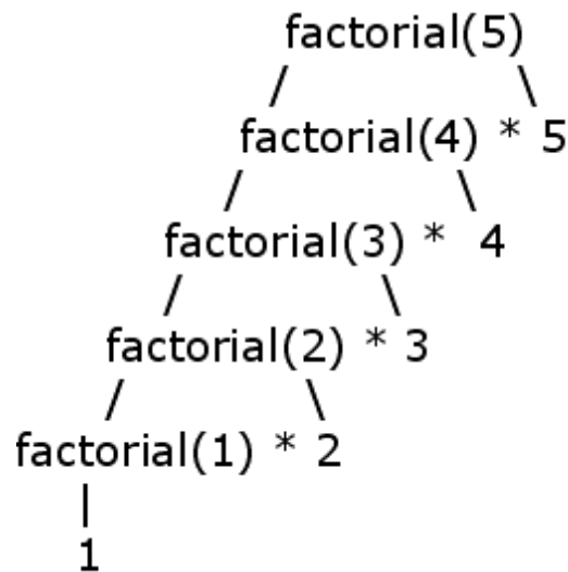
Gambar 1: Contoh Factorial
